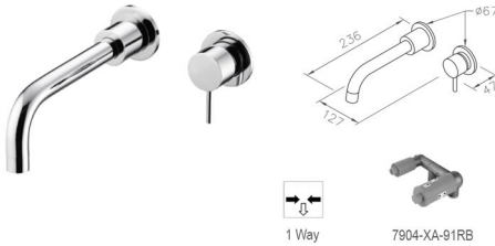
6771-X2-80CP Wall-Mounted Basin Mixer
