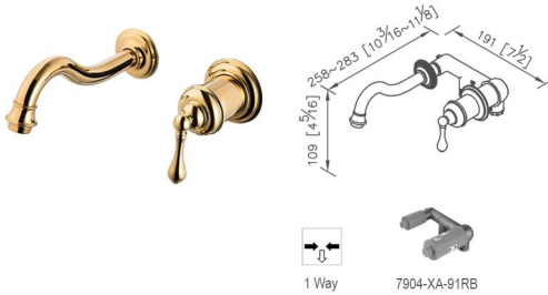
6703-X2-80PK Wall-Mounted Basin Mixer
