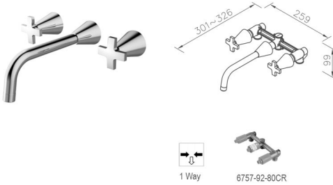
7874-92-81CP Wall-Mounted Basin Mixer
