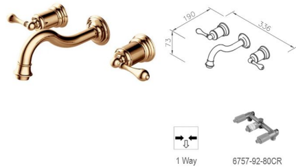
9703-92-80PK Wall-Mounted Basin Mixer
